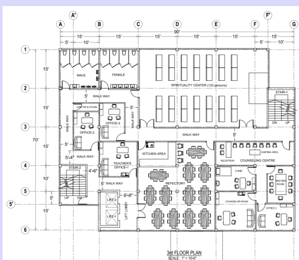
3rd Floor with Spirituality Center
